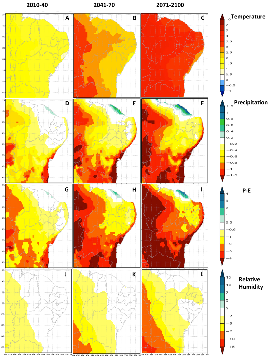
Fig. 2 Changes in annual air temperature ( ^{\circ}\text{C} , a-c ), rainfall ( \text{mm day}^{-1} , d-f ), precipitation-evaporation ( \text{mm day}^{-1} , g-i ) and relative humidity ( \% , j-l ), derived from the downscaling of the HadCM3 models using the 40 km lat-lon Eta regional model, A1B scenario. Left column is for 2010–40, center column for 2041–70 and right column for 2071–2100. Changes are relative to 1961–90. Color scale is on the right side of the panel
